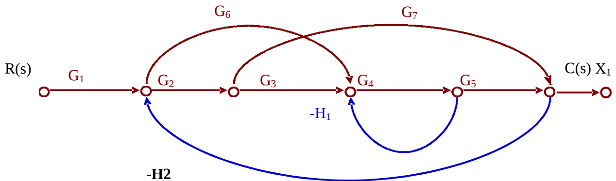
Figure 3 Signal flow graph of example 3
