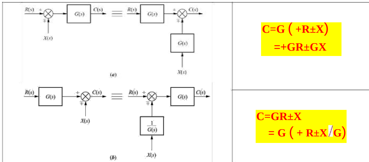
Figure 10.4 Summing junctions.
