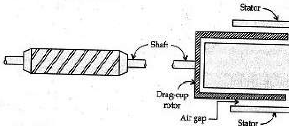
Fig. 9.5 (a) Squirrel cage rotor
