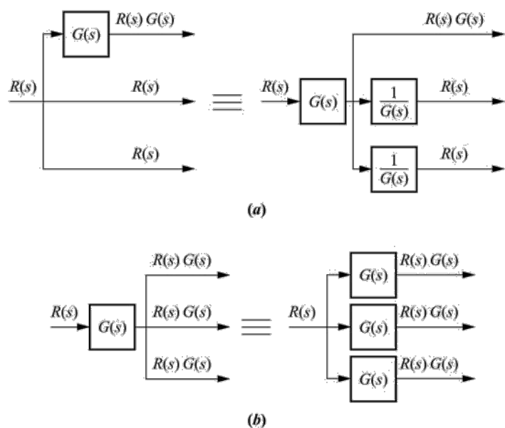
Figure 10.5 Summing junctions.
