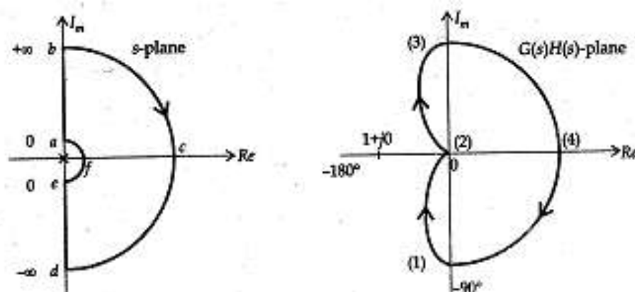
Fig. 5.42. Nyquist plot
