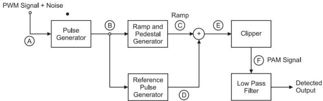
PWM Detector
