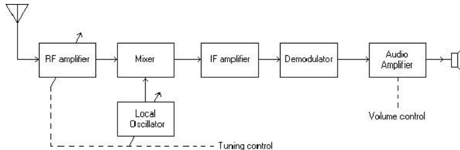
Super-Heterodyne Receiver
