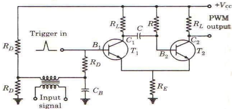
Monostable multivibrator generating pulse width modulation (PWM).
