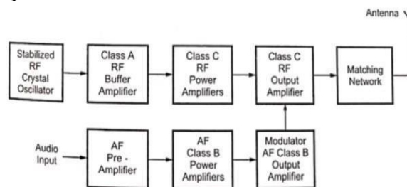
Block Diagram of High Level Modulation
