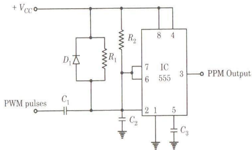
PPM Generator
