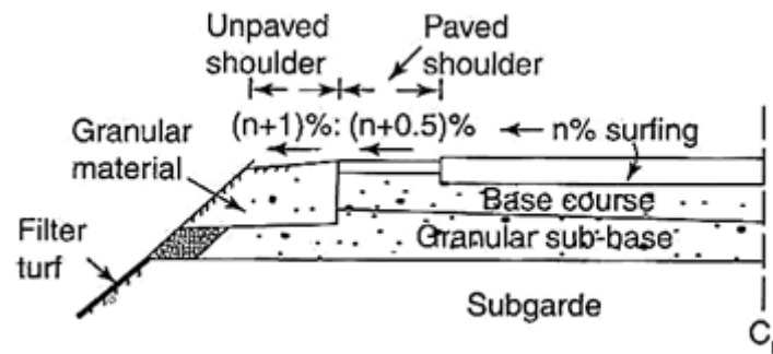
Fig. Shoulder Drainage
