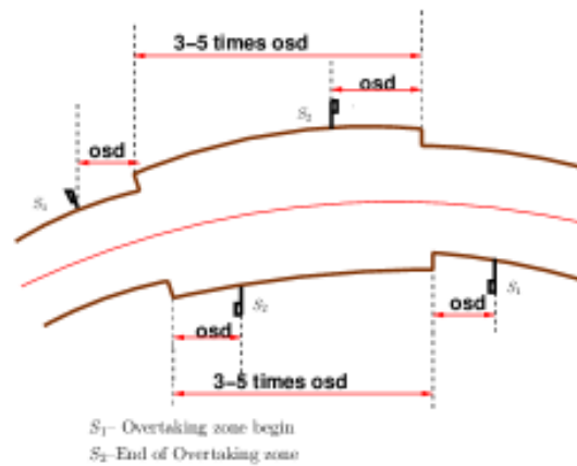
Figure : Overtaking zones
