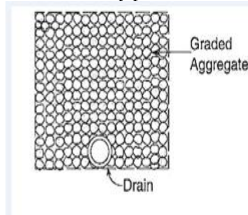
Fig. Geosynthetic-encased aggregate drain with a pipe
