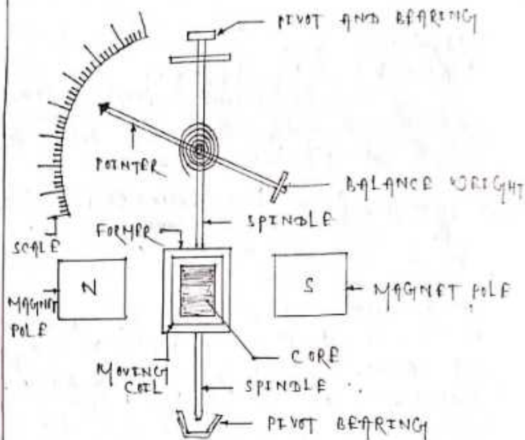
(Fig: PMMC type instrument)
