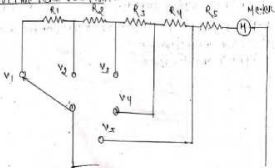
Fig: block diagram of multimeter
