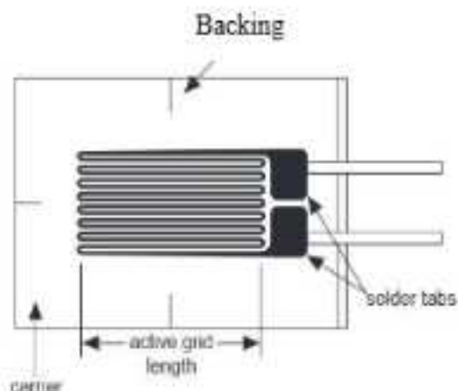
Figure: Wire type bonded strain gauge
