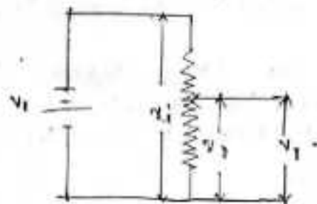
(Fig-1 Linear potentiometer)
