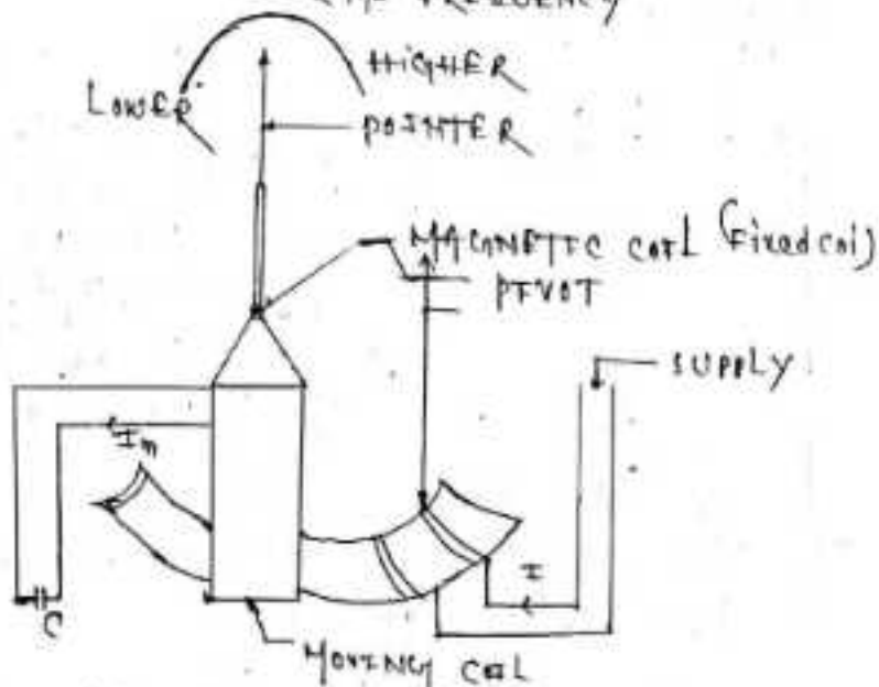
Fig: Ferrodynamic electrical resonance frequency meter.
