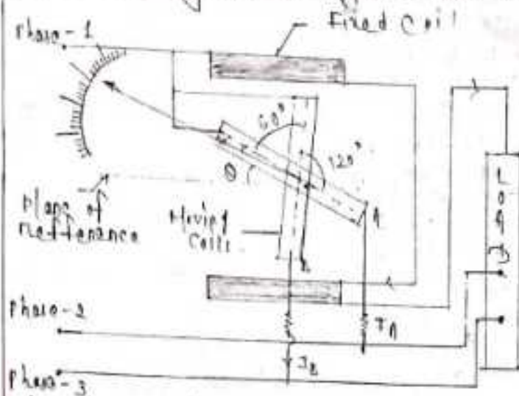
(Fig. 3- \phi Electro-dynamometer type power factor meter)
