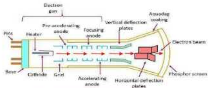
Internal structure of CRT
