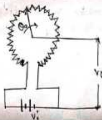
(Fig-2 Angular potentiometer)
