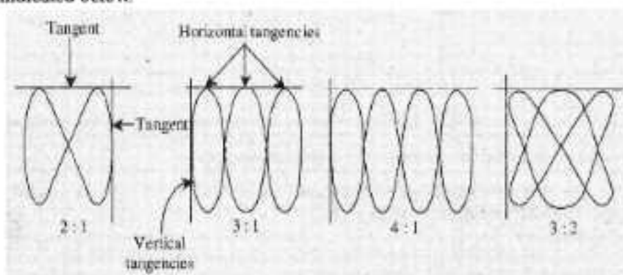
Fig 6.2 Lissajous patterns showing different frequency ratios.
