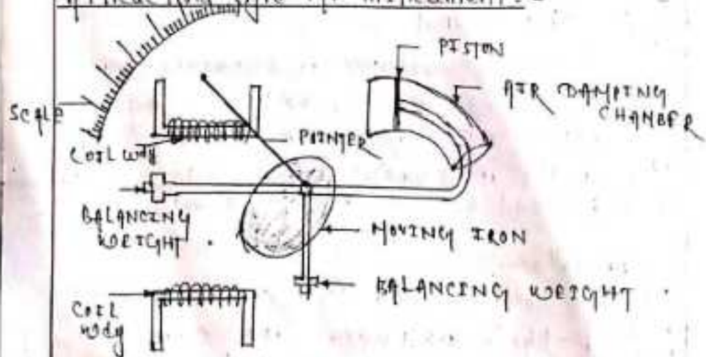
(Fig: Attraction type MI instrument)
