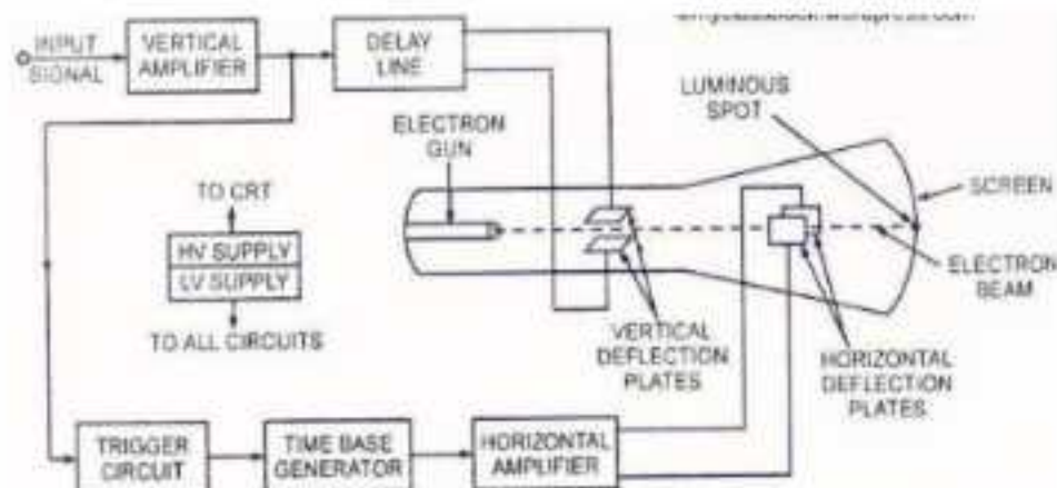
Figure: Block diagram of CRO
