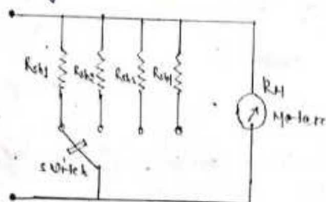
(Fig: Multi-range ammeter)
