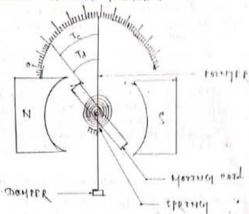
(Fig: PMMC type indicating instrument)
