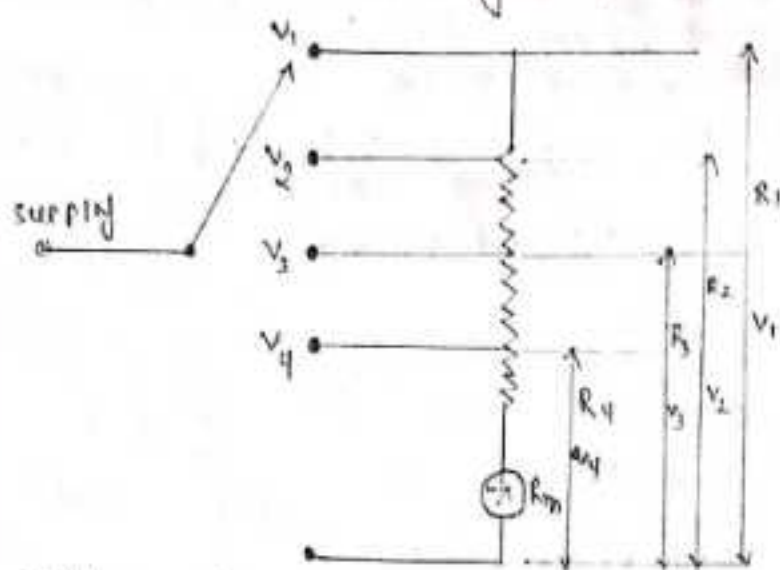
Fig: Multirange voltmeter using potential divider arrangement.
