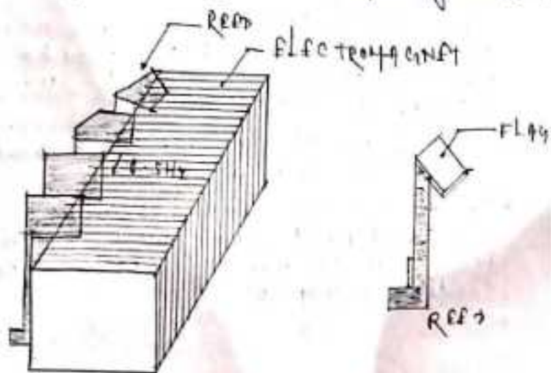
(Fig: vibrating reed type frequency meter)
